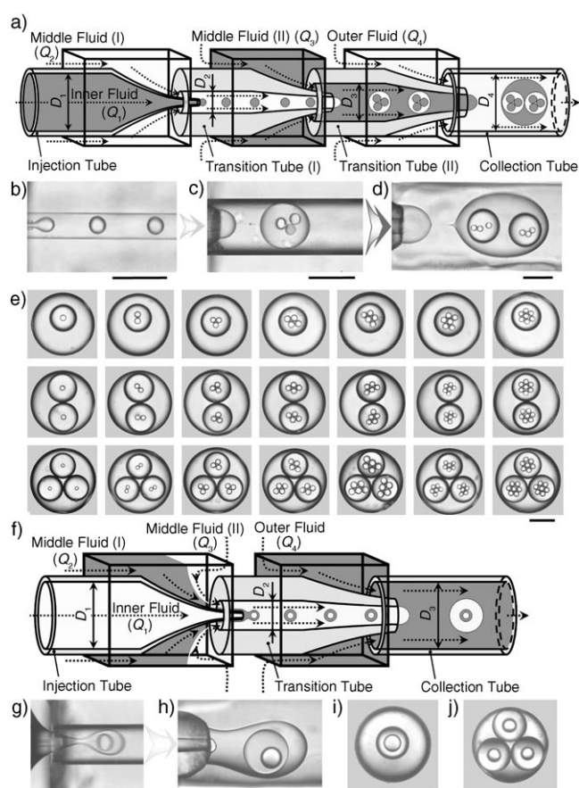
Figure 3. Generation of highly controlled monodisperse triple emulsions. a) Schematic diagram of the extended capillary microfluidic device for generating triple emulsions. b)–d) High-speed optical micrographs displaying the first (b), second (c), and third (d) emulsification stages. The flow rates of the inner, middle (I), middle (II), and outer fluids in (b)–(d) are Q_1=50 , Q_2=500 , Q_3=2000 , and Q_4=5000 \mu\text{L h}^{-1} . e) Optical micrographs of triple emulsions that contain a controlled number of inner and middle droplets. The variation ranges for the flow rates are Q_1 \approx 5 –100, Q_2 \approx 200 –1000, Q_3 \approx 2000 –3500, and Q_4=5000 \mu\text{L h}^{-1} . f) Schematic diagram detailing an alternate method for generating triple emulsions where the middle fluid (II) is injected from the entry side of the first square tube, leading to flow-focusing of the first middle fluid into the transition capillary. g) and h) High-speed optical micrographs showing the formation of double emulsions in a one-step process in the transition capillary (g) and the subsequent formation of triple emulsions in the collection capillary (h). i) and j) Optical micrographs of triple emulsions that contain a different number of double emulsions. The variation ranges for the flow rates in (g)–(j) are Q_1=50 –200, Q_2=1600 –2500, Q_3=4000 –8000, and Q_4=5000 –12 000 \mu\text{L h}^{-1} . The scale bar in all images is 200 \mu\text{m} .
